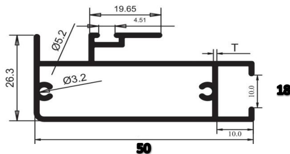
R.C-45001 INTERLOCK
