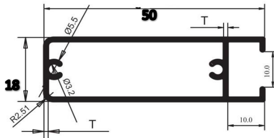
R.C-44001 HANDLE
