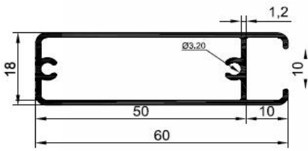
RC-43001 HANDLE
